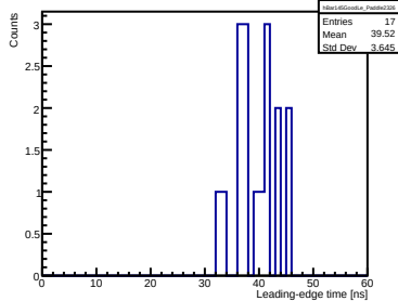
Bar 145, Paddle 2330
