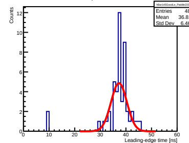
Bar 145, Paddle 2335
