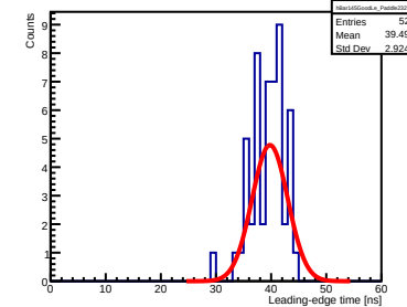
Bar 145, Paddle 2331
