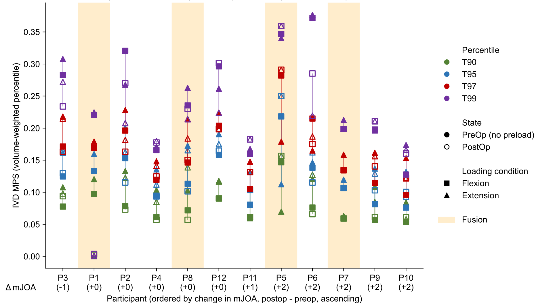
IVD strain (T90/T95/T97/T99): PreOp (no preload) vs PostOp, by fusion status
