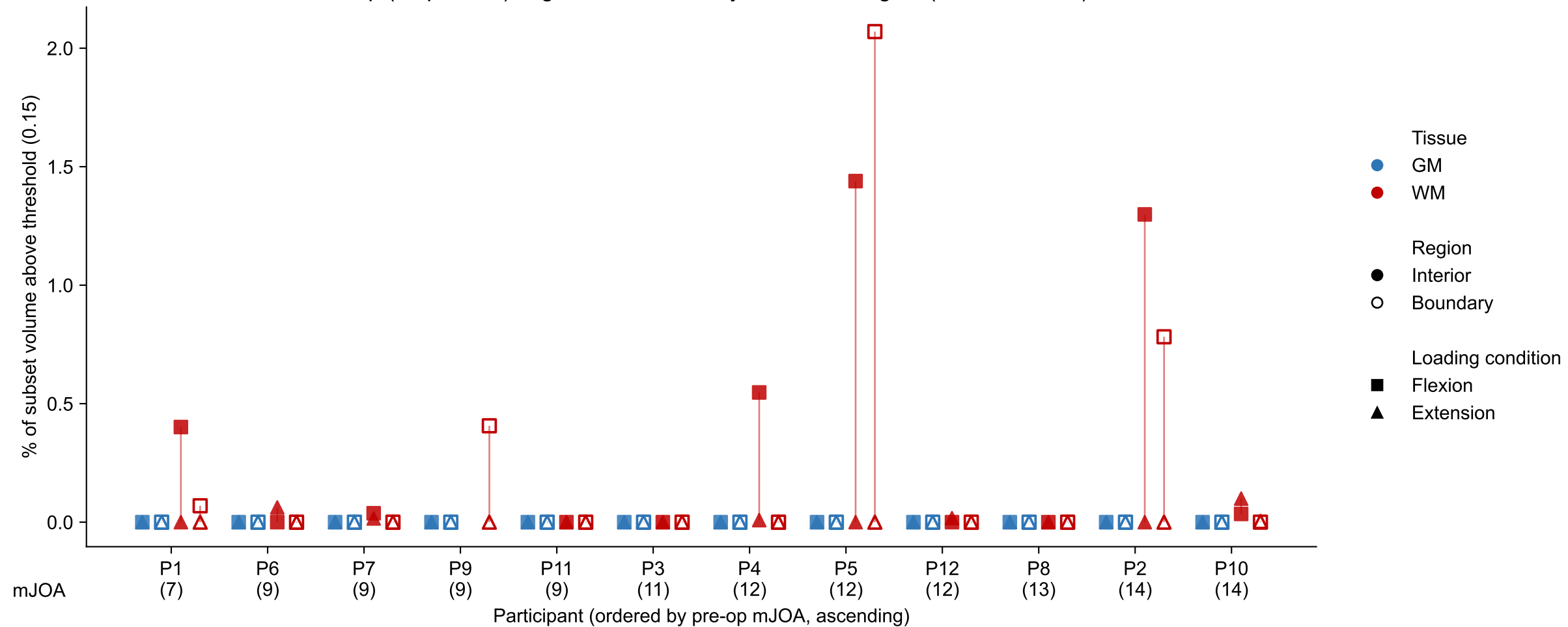
PreOp (no preload): high-strain volume by tissue and region (threshold 0.15)
