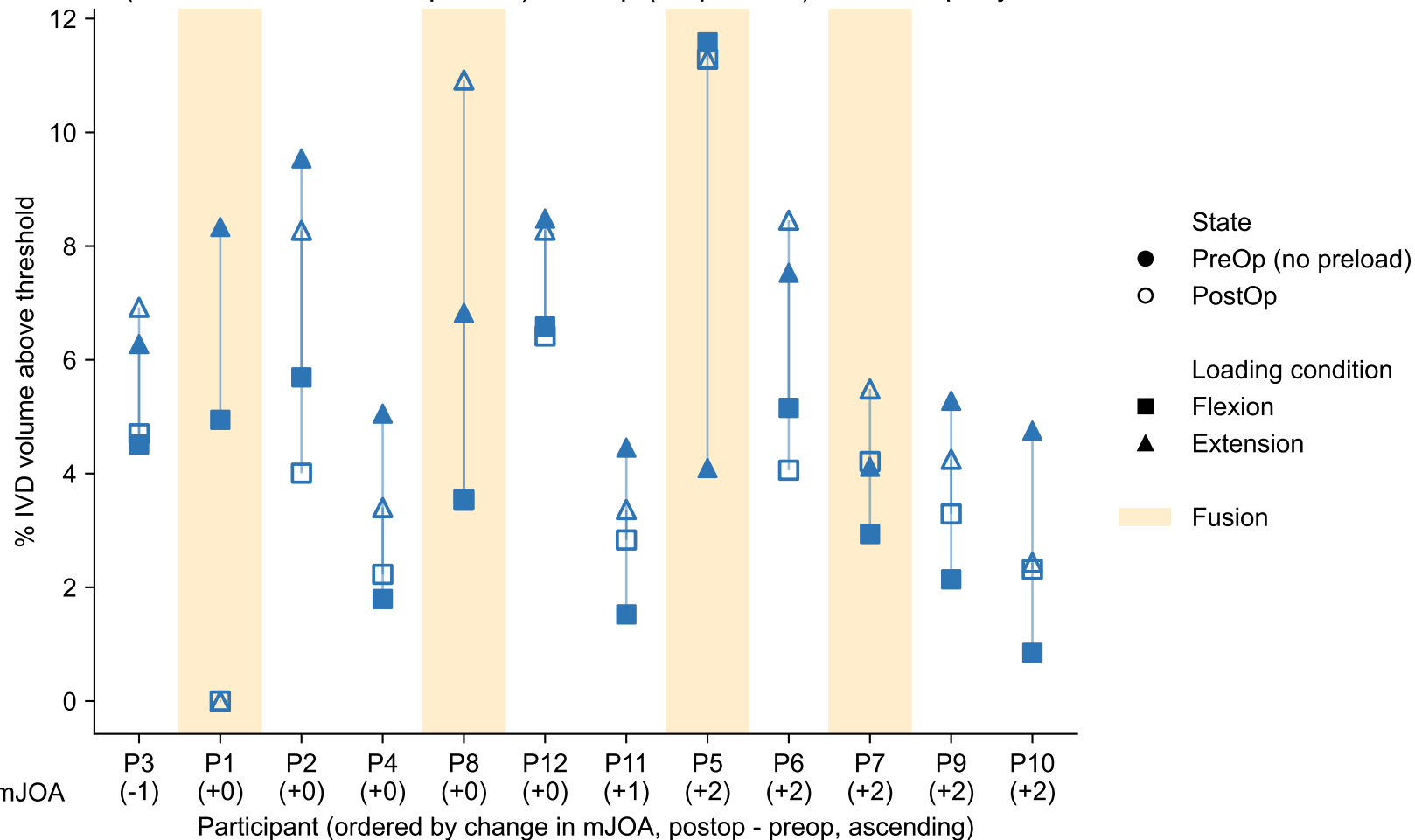
IVD strain (T95 = 0.1350, cohort-pooled): PreOp (no preload) vs PostOp, by fusion status
