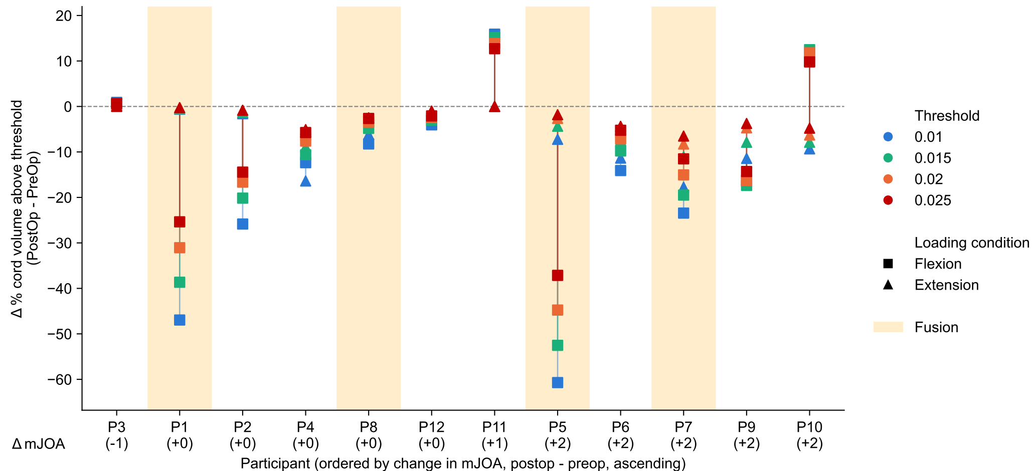
\Delta\% cord volume above MPS threshold (PostOp - PreOp no preload), by operation type
