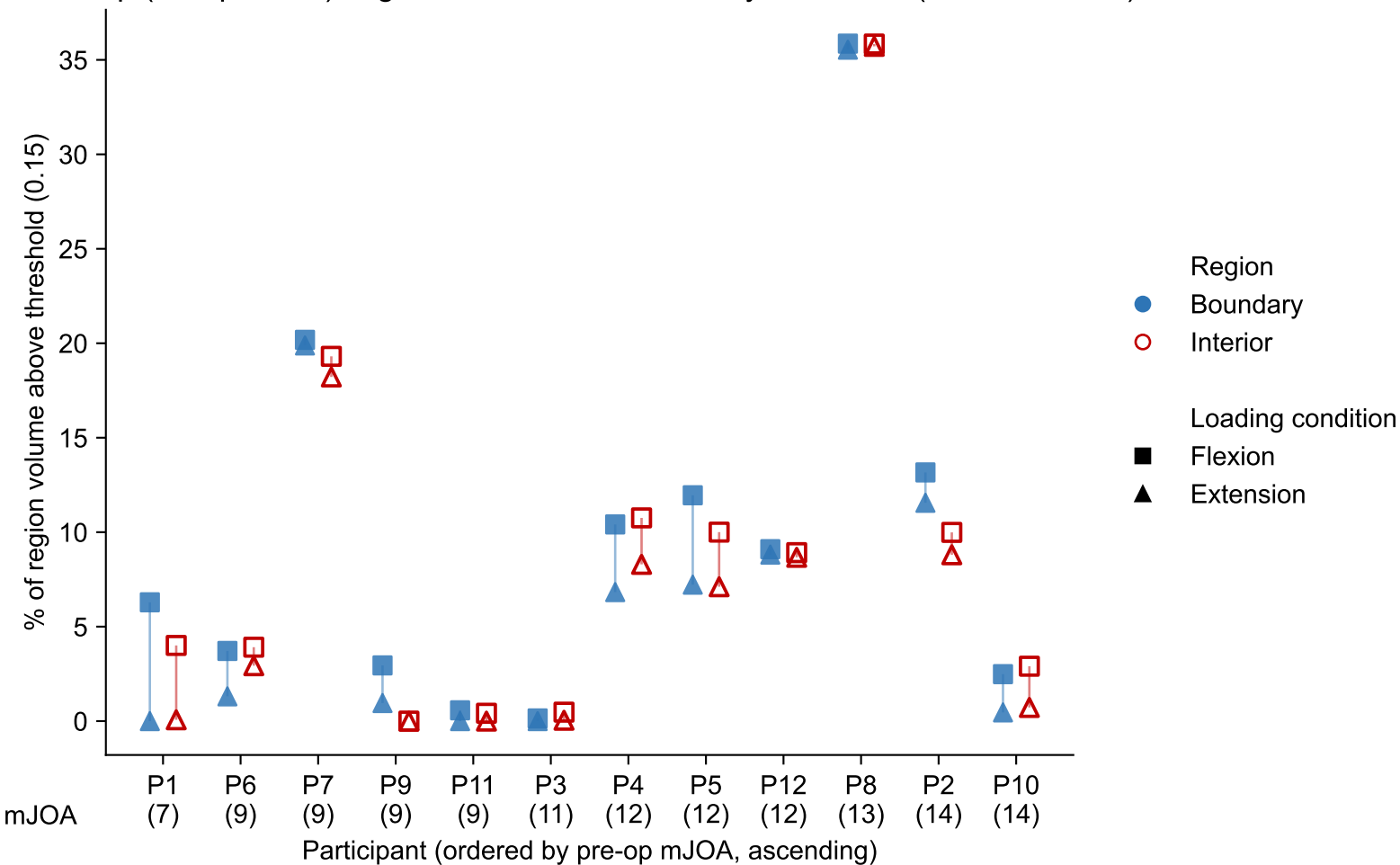
PreOp (with preload): high-strain volume, boundary vs interior (threshold 0.15)
