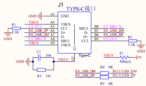
Type C-USB 供电 STM32-USB Slave
