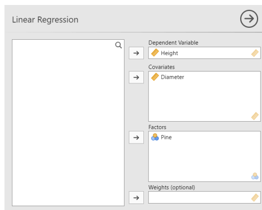
Figure 9.5: Adding a binary variable
