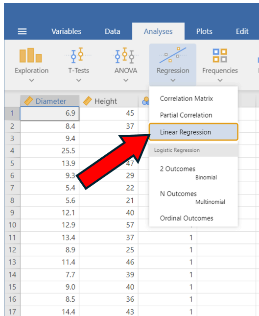
Figure 9.3: Select 'Linear Regression'
