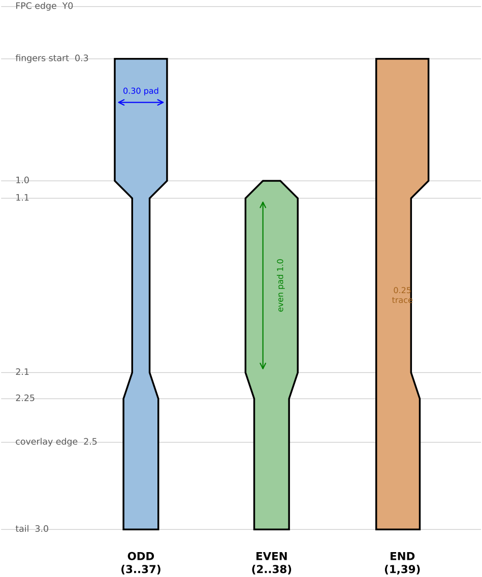
Finger profiles (mm) — Y0 = FPC edge, +Y toward ribbon
