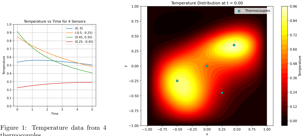
Figure 2: Reconstructed temperature field at one time step.
