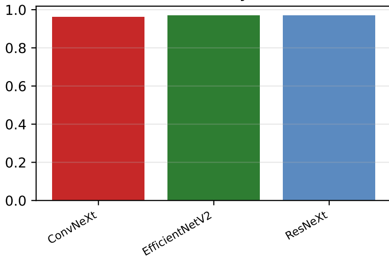
Recall (macro)
