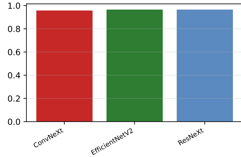
MCC
