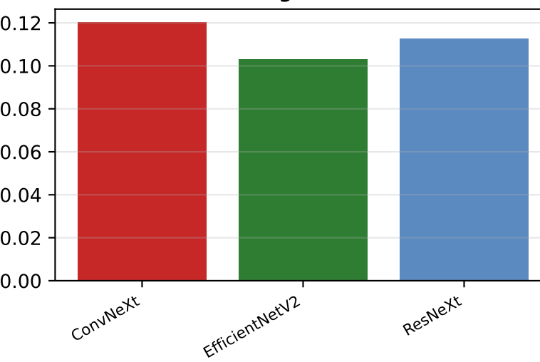
Avg. Loss
