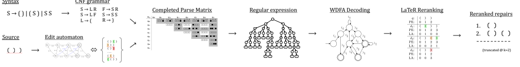
Fig. 1. Tidyparse represents the bounded edit neighborhood as an automaton, intersects it with the language grammar, and compiles the finite intersection into a generalized regular expression. A probabilistic decoder enumerates likely members, which a learned model reranks for presentation.
