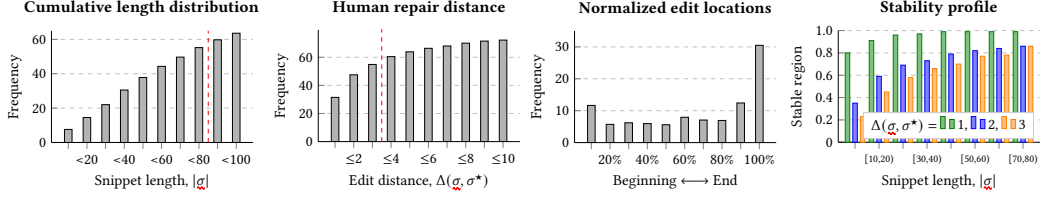
Fig. 12. Repair statistics across the Stack Overflow dataset. Tidyverse can handle about 90% in under \sim 1 s and \sim 4 GB. Larger repairs and edit distances are possible, albeit requiring additional time and memory.
