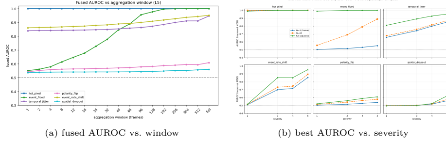
Figure 5: Aggregation and severity. (a) Fused AUROC vs. pooling window per corruption. (b) Improved-MDD AUROC vs. severity at W = 1 / 64 / \text{full sequence} . Source: plot_corruption_graphs.py.
