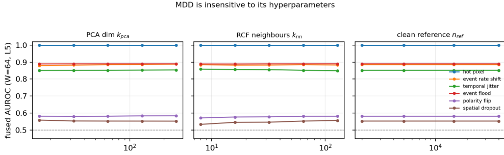
Figure 12: MDD hyperparameter sensitivity (fused AUROC, W=64 , L5 ). Every corruption’s curve is essentially flat across k_{pca} , k_{nn} , and n_{ref} ( \log x ), with the only visible movement on the two residuals at very small k_{nn} . Source: plot_new_graphs.py ( mdd_sensitivity.csv ).
