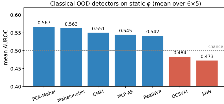
Figure 11: Seven classical OOD detectors on static \varphi , mean AUROC over all corruptions/severities. PCA-Mahalanobis/Mahalanobis lead; k NN/OCSVM invert below chance on the contractions – one-sided detectors cannot face both ways, motivating MDD. Source: plot_appendix_graphs.py (ood_metrics.csv).
