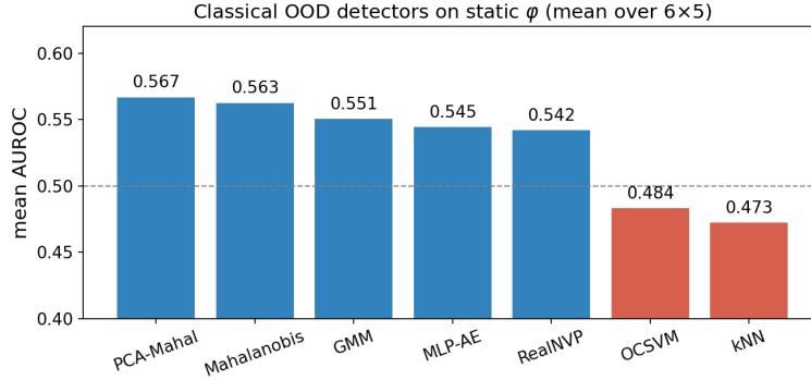
Figure 11: Seven classical OOD detectors on static \varphi , mean AUROC over all corruptions/severities. PCA-Mahalanobis/Mahalanobis lead; kNN/OCSVM invert below chance on the contractions – one-sided detectors cannot face both ways, motivating MDD. Source: plot_corruption_graphs.py (ood_metrics.csv).
