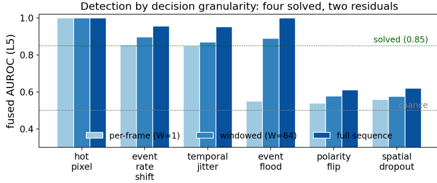
Figure 6: Detection by decision granularity (L5). Per-corruption fused AUROC at three granularities – per-frame ( W=1 ), a bounded 64-frame window, and full recording. Four corruptions cross the 0.85 “solved” line (hot_pixel/event_rate_shift/temporal_jitter already per frame, event_flood with a short window); polarity_flip and spatial_dropout are the two residuals near chance at every granularity. The whole result in one view. Source: plot_corruption_graphs.py (final_results.csv).
