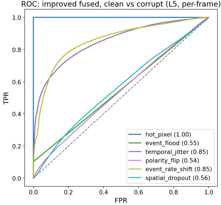
Figure 3: ROC curves of the improved fused MDD at L5 (per-frame), clean vs. each corruption. Source: plot_corruption_graphs.py ( 18_roc_curves_L5 ).
