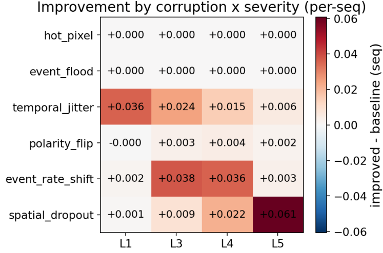
Figure 8: Improved – baseline per-sequence AUROC, per corruption \times severity. Source: plot_corruption_graphs.py (22_improvement_by_severity).
