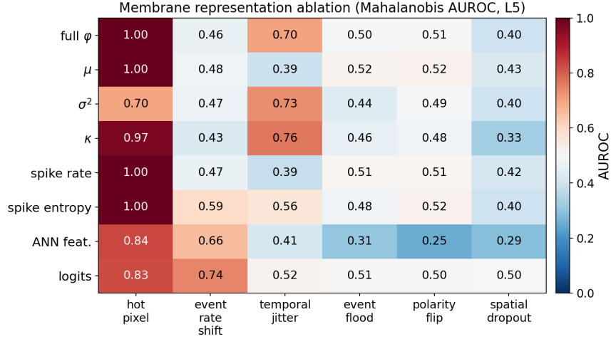
Figure 10: Membrane representation ablation (Mahalanobis AUROC, L5). \sigma^2/\kappa carry temporal_jitter while \mu /spike-rate do not; ANN features are the weakest overall and collapse on contractions/polarity. Source: plot_corruption_graphs.py.
