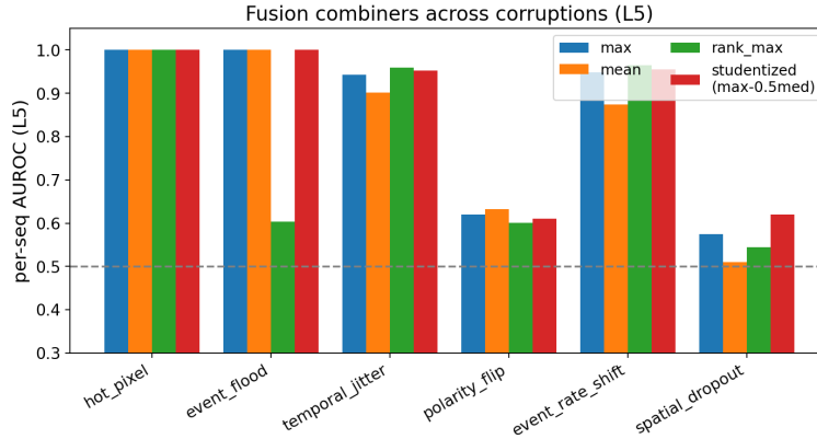
Figure 9: Fusion-combiner sweep across corruptions (per-sequence, L5). Source: plot_corruption_graphs.py (17_fusion_combiners).
