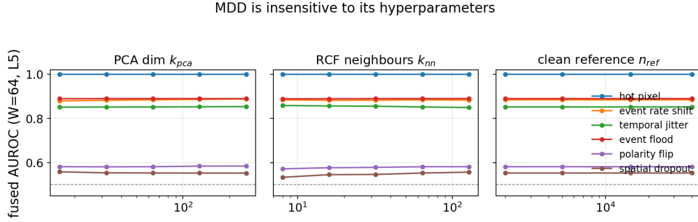
Figure 12: MDD hyperparameter sensitivity (fused AUROC, W=64 , L=5 ). Every corruption’s curve is essentially flat across k_{pca} , k_{nn} , and n_{ref} ( \log x ), with the only visible movement on the two residuals at very small k_{nn} . Source: plot_corruption_graphs.py ( mdd_sensitivity.csv ).
