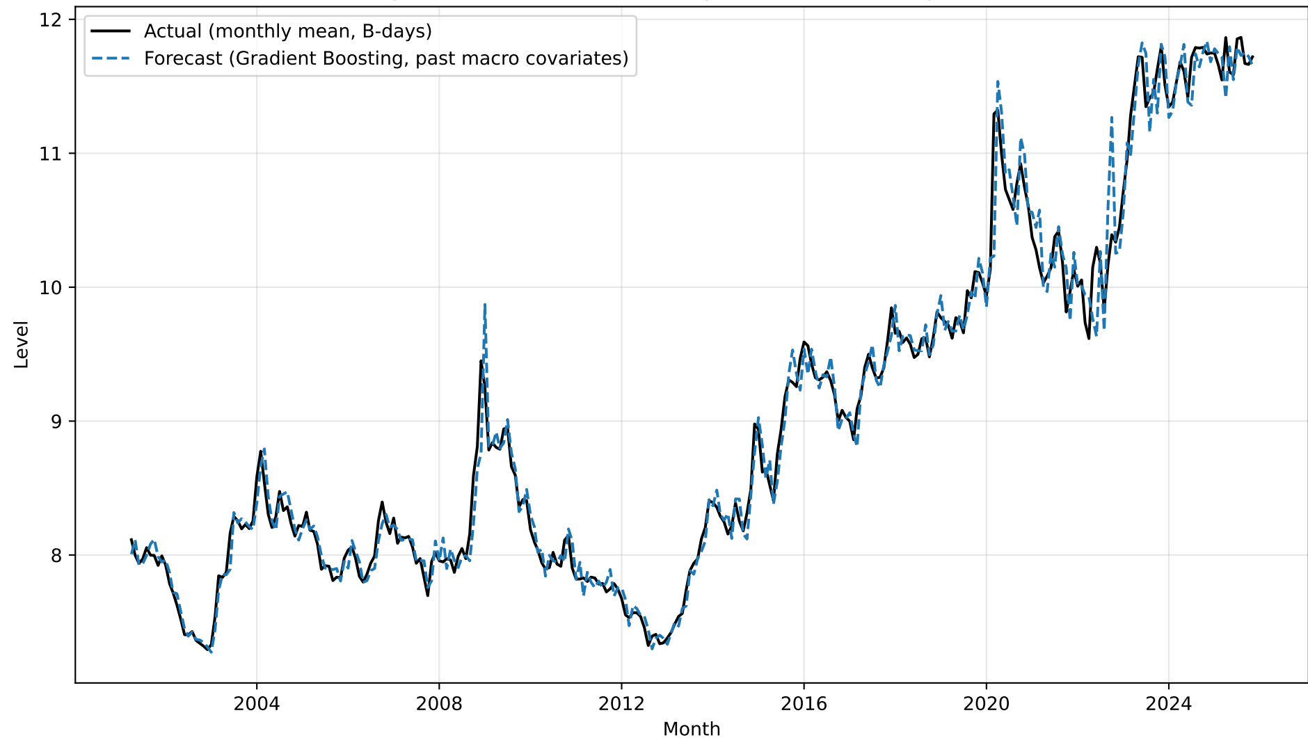
Gradient Boosting Forecast vs Actual (Monthly Mean, EUR/NOK - past macro covariates)
