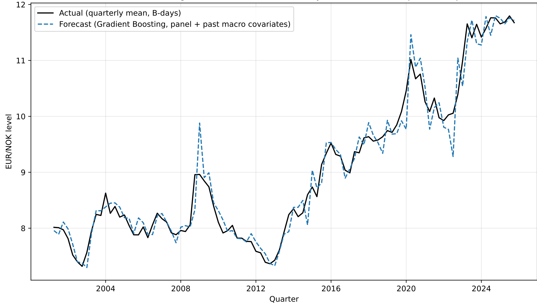
Gradient Boosting Forecast vs Actual (Quarterly Mean, EUR/NOK - panel setup)
