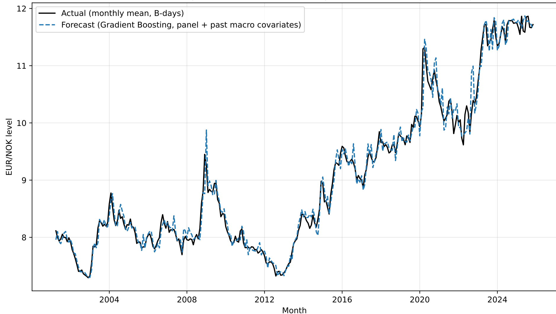
Gradient Boosting Forecast vs Actual (Monthly Mean, EUR/NOK – panel setup)
