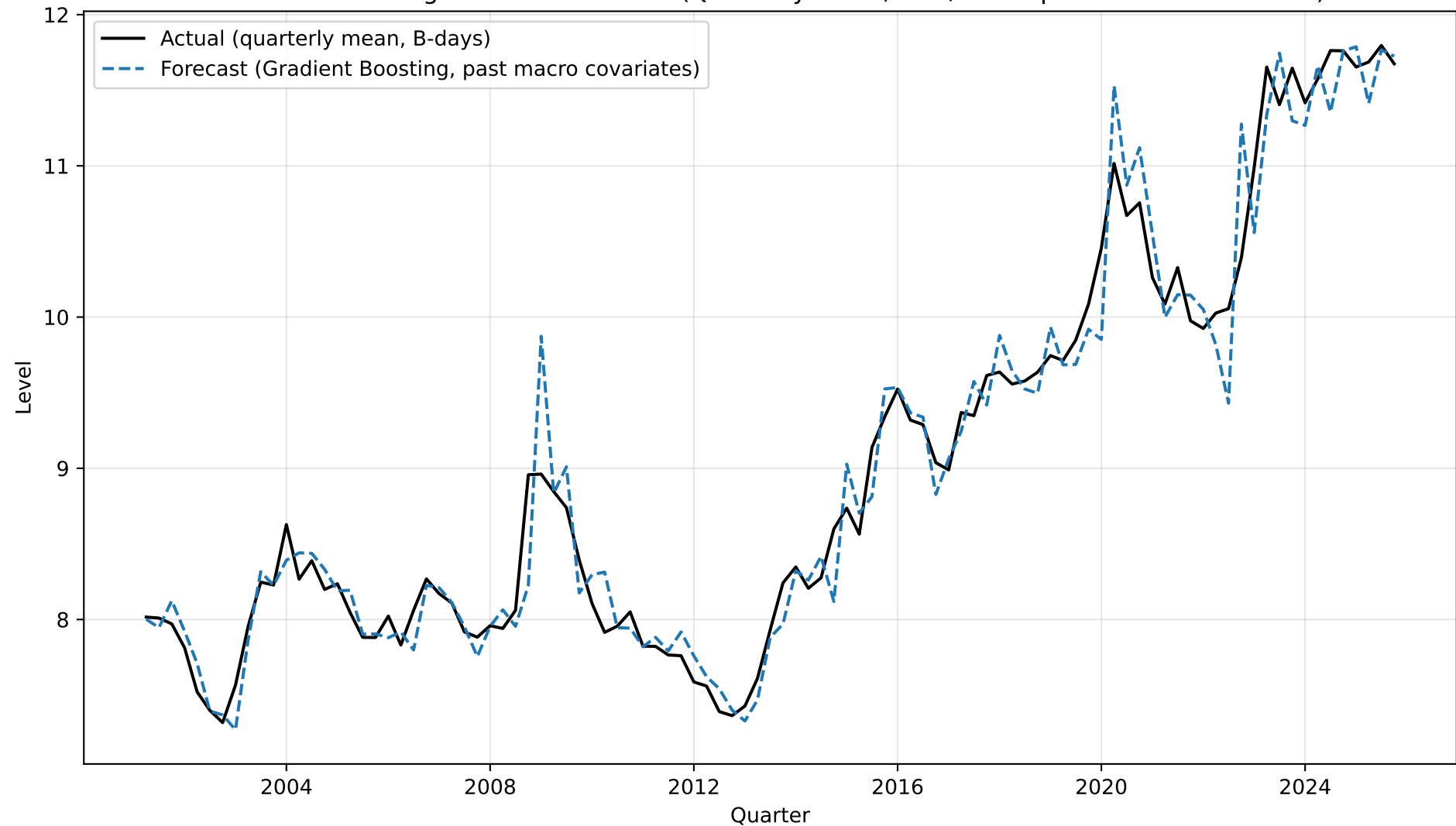
Gradient Boosting Forecast vs Actual (Quarterly Mean, EUR/NOK – past macro covariates)
