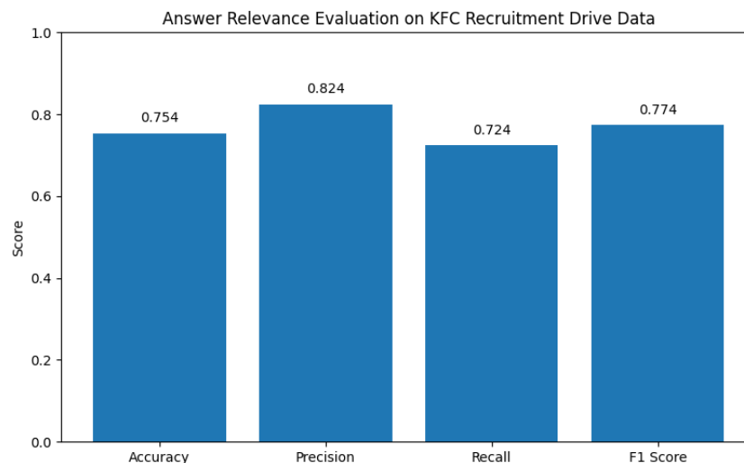
Figure 5.10: Evaluation metrics for the answer relevance module on KFC recruitment drive video data.
