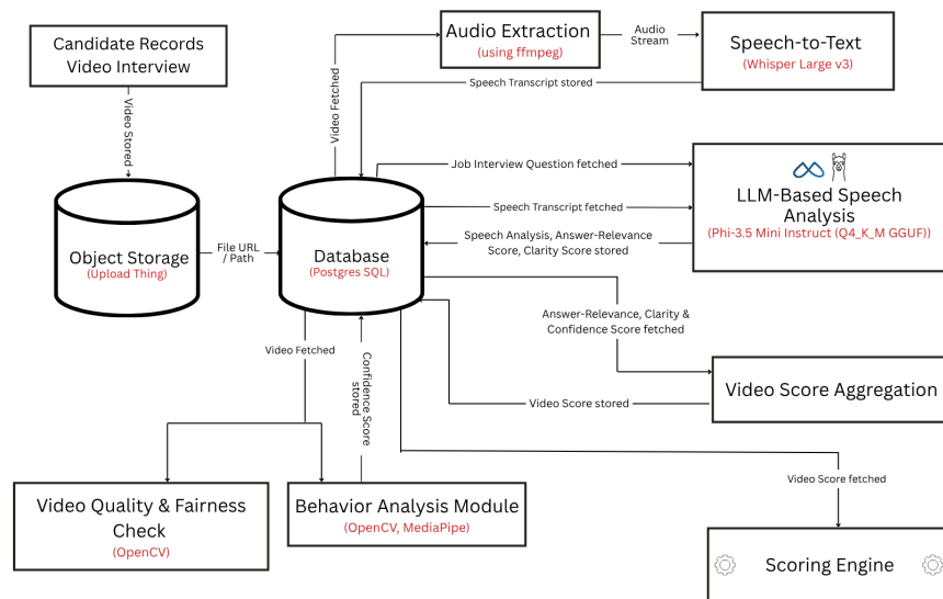
Figure 4.4: Video Processing Pipeline
