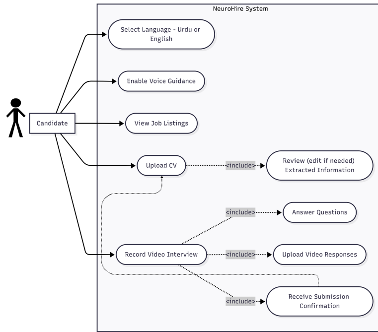
Figure 3.2: Candidate Use Case Diagram
