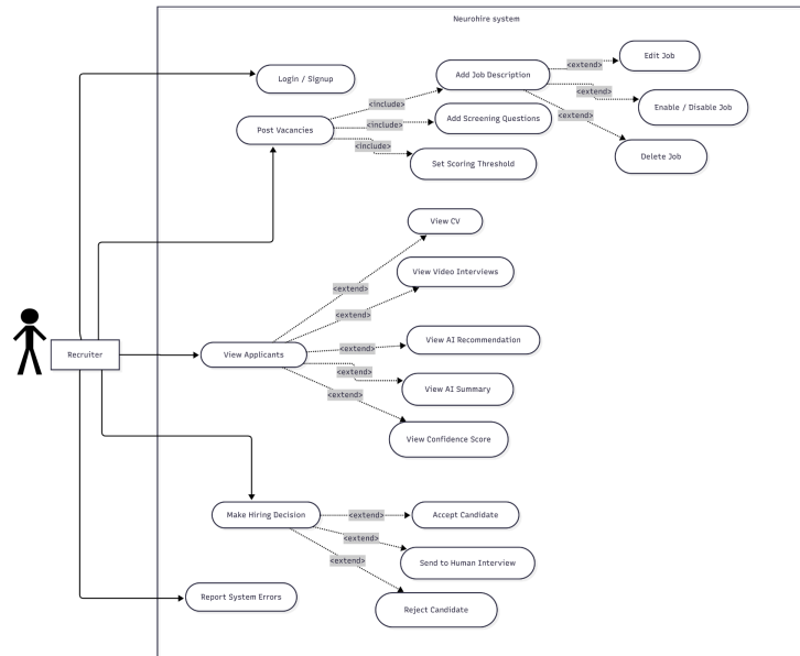
Figure 3.3: Recruiter Use Case Diagram
