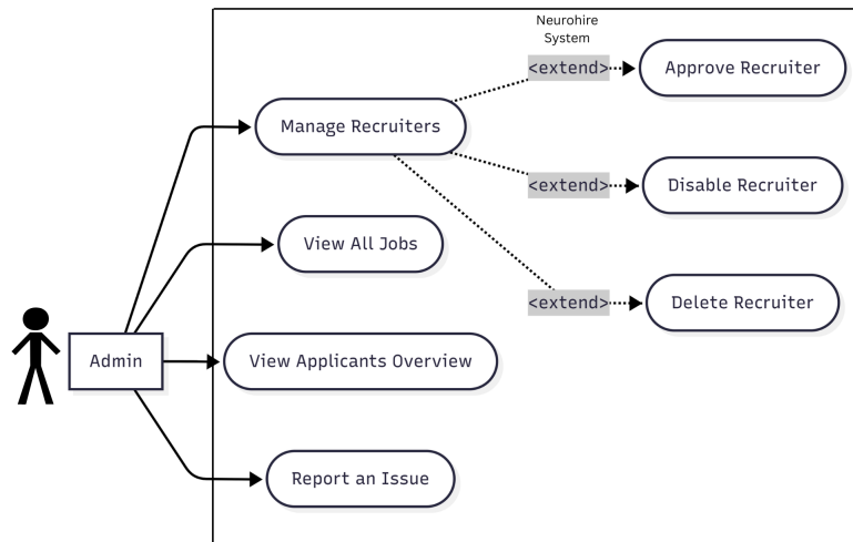
Figure 3.4: Admin Use Case Diagram
