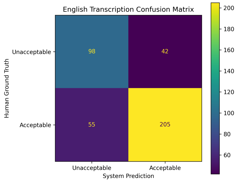
Figure 5.4: Confusion matrix for English transcription evaluation.
