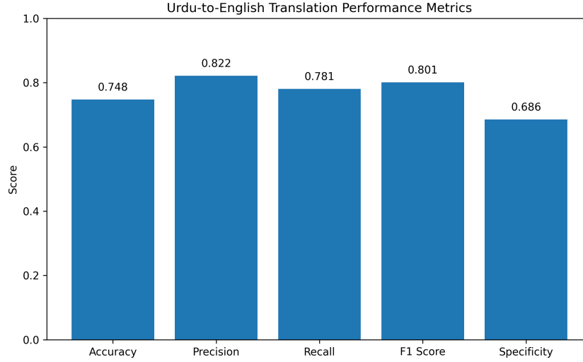
Figure 5.7: Performance metrics for Urdu-to-English translation evaluation.
