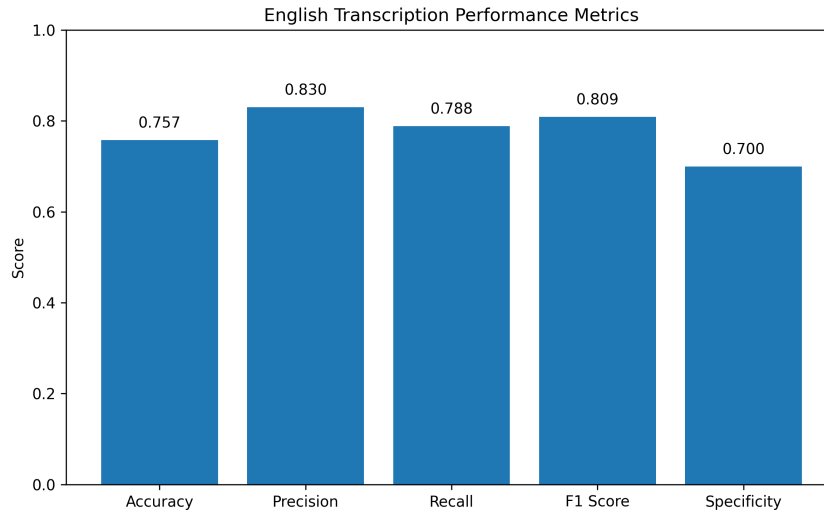
Figure 5.5: Performance metrics for English transcription evaluation.
