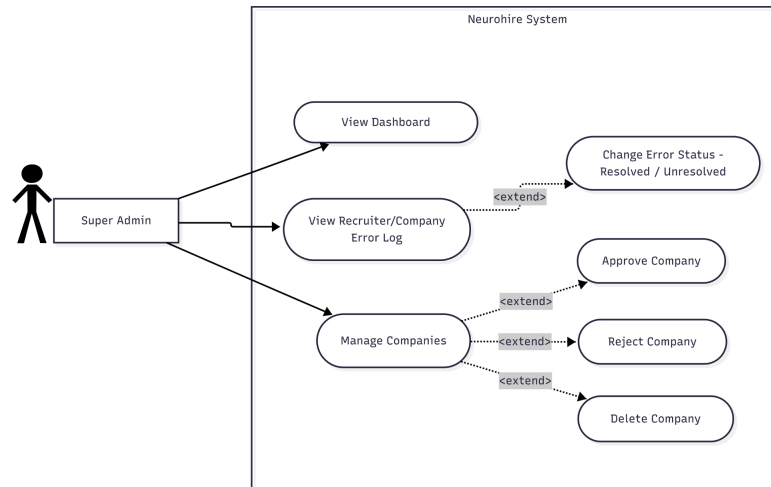
Figure 3.5: Super Admin Use Case Diagram
