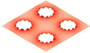
Figure 4.4: A simulation of the Schnakenberg equations with extra decay for v on \Omega = (-8, 8)^2 with \delta_v = 0.1 , d = 50 , a = 0.1 , b = 0.9 and \gamma = 12 . The solution is plotted for times t = 0 , t = 5/\gamma and t = 11/\gamma .
