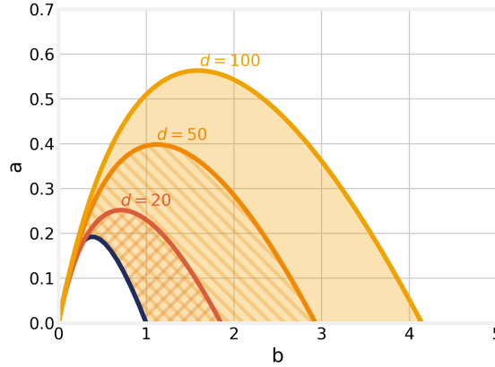
Figure 2.1: The Turing space for Equation (2.4) plotted for d = 20 , d = 50 and d = 100 .
