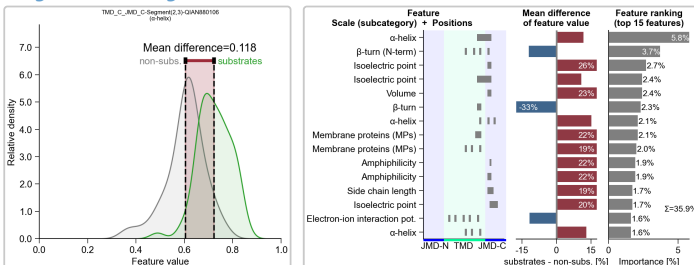
CPPPlot.feature · top feature
