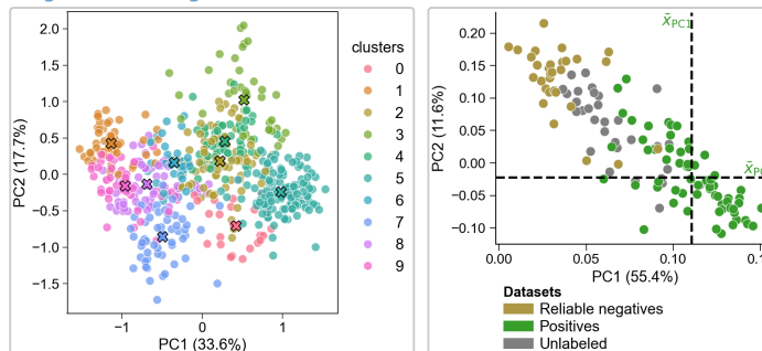
AAclustPlot.centers · cluster scale profiles
