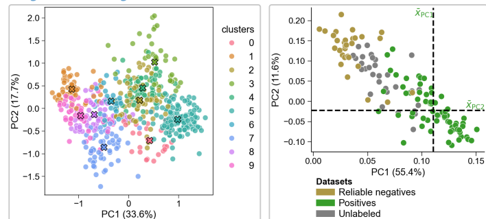
AAclustPlot.centers · cluster scale profiles
