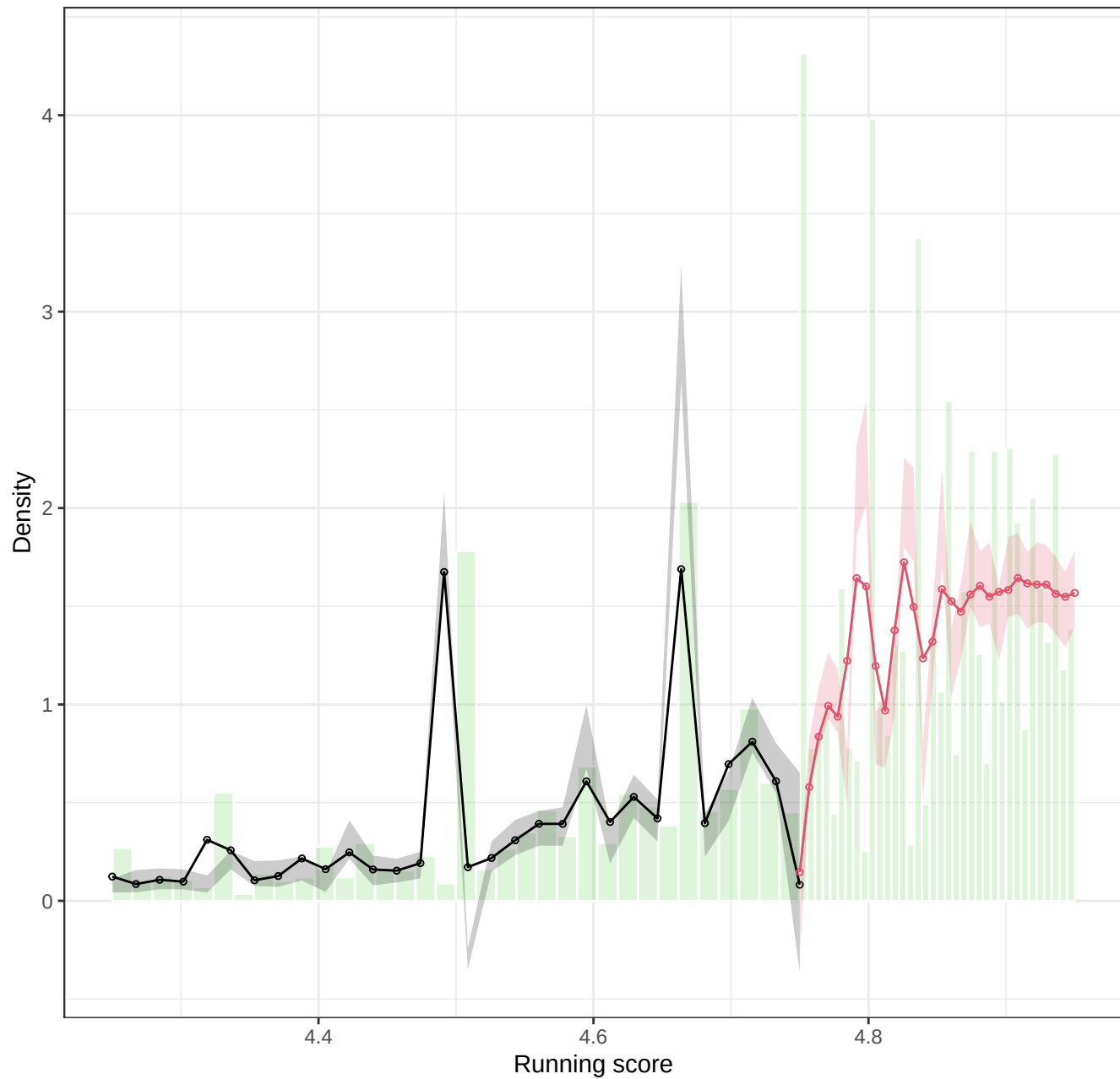
McCrary density test at the true cutoff (4.75)
