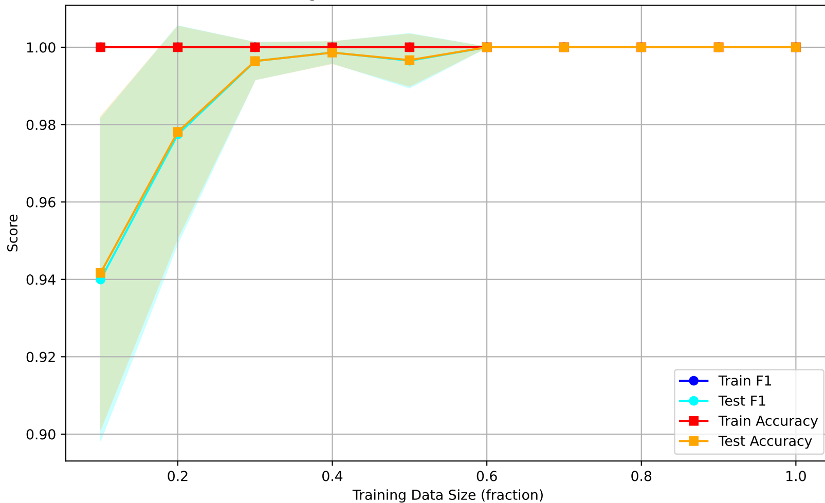
Learning Curve with Error Bands (RandomForest)
