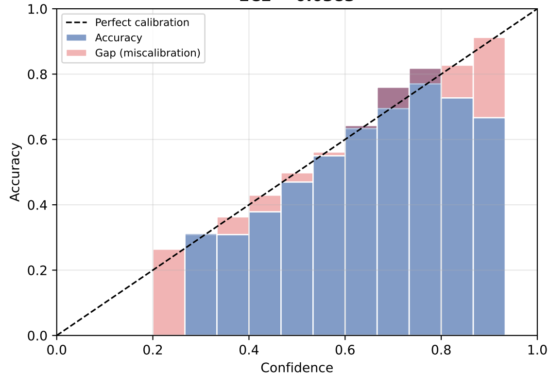
Pipeline B — QLoRA ECE = 0.0383
