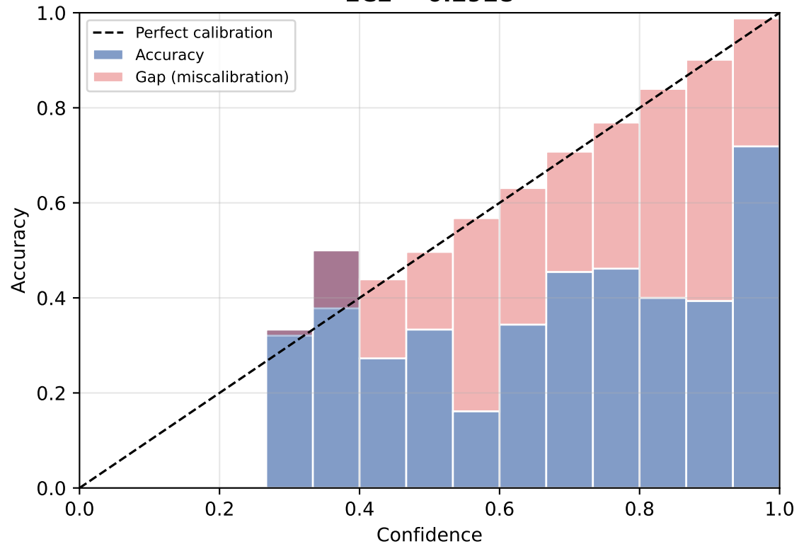
Pipeline A — PTQ ECE = 0.2928
