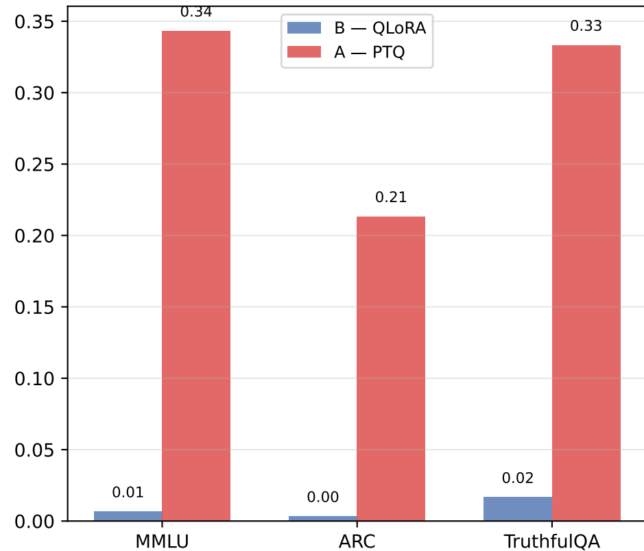
Overconfidence Rate
