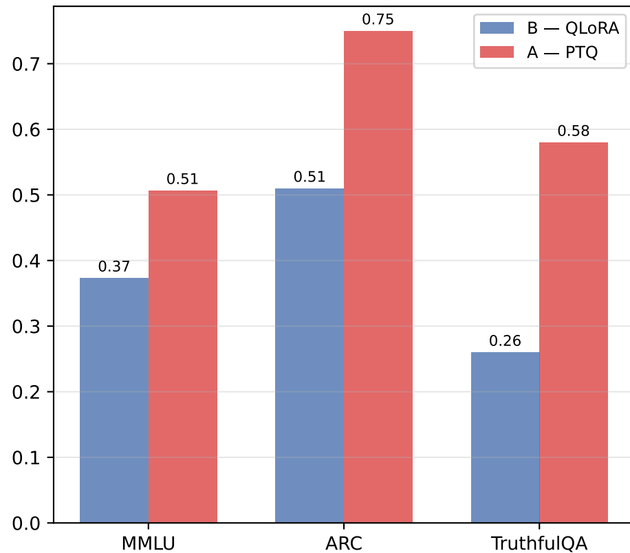
Accuracy
