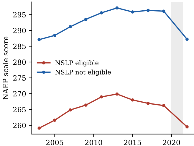
Math, Grade 8
