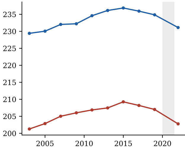
Reading, Grade 4
