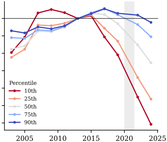
Reading, Grade 4
