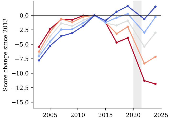
Math, Grade 4
