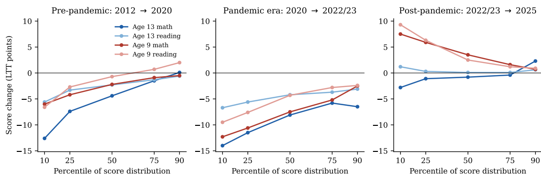
Figure 4: LTT score changes by percentile in three windows: pre-pandemic (left), pandemic era (center), post-pandemic (right). The pre-pandemic decline is concentrated almost entirely among low performers; the pandemic-era decline hits everywhere but is steepest at the bottom; after 2022/23 the recovery is bottom-led at age 9, while at age 13 the bottom of the mathematics distribution keeps falling as the top recovers. Data: LTT Data Service.
