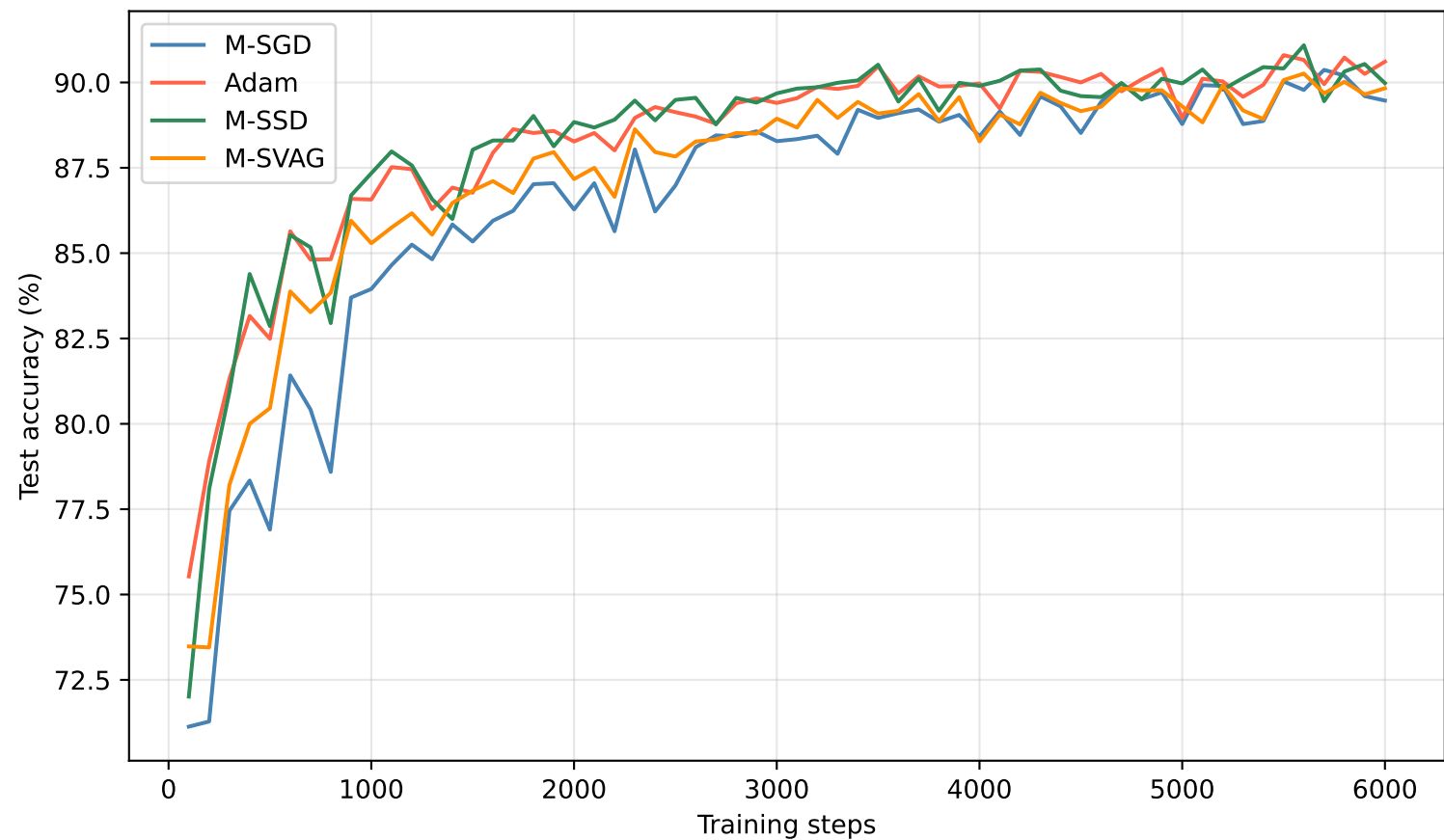
Fashion-MNIST — 10 seeds, mean \pm 1 std
