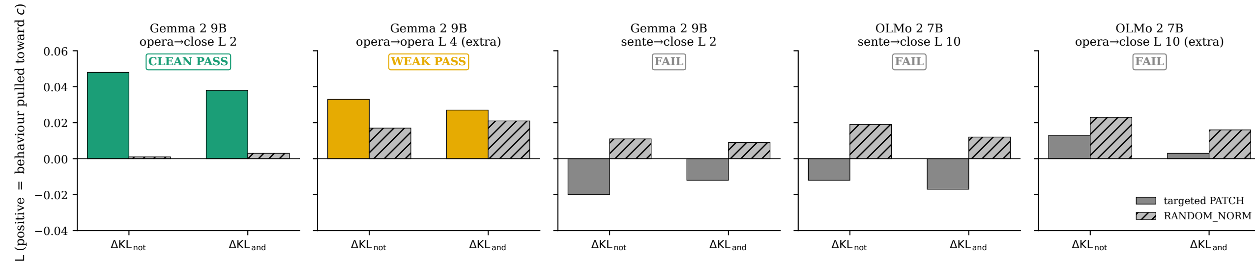
Figure 4. Causal patching across 5 (source, target, layer) cells. Targeted PATCH (coloured) vs. norm-matched RANDOM_NORM control (grey, hatched), per reference axis. A cell is causally arity-respecting only when targeted \Delta\text{KL} clearly exceeds RANDOM_NORM on the same axis. (extra) = reviewer-round-1 follow-up cell.
