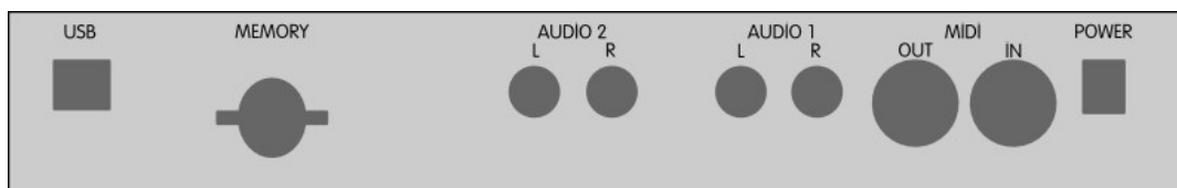
Figure 2. LXR rear panel connections.
