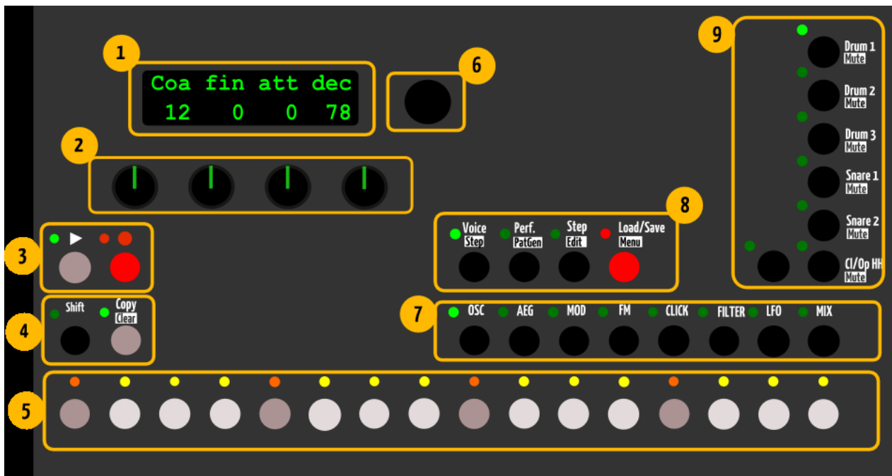
Figure 8. Front panel reference for using Voice mode.
