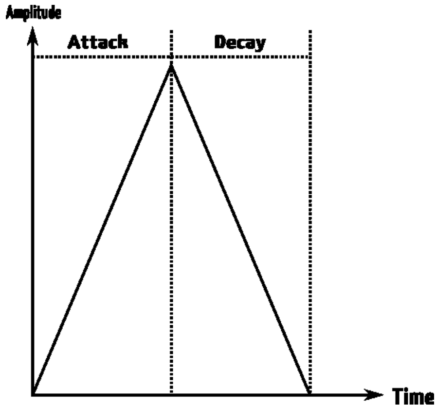
Figure 18. Linear envelope curve (slope = 63).
