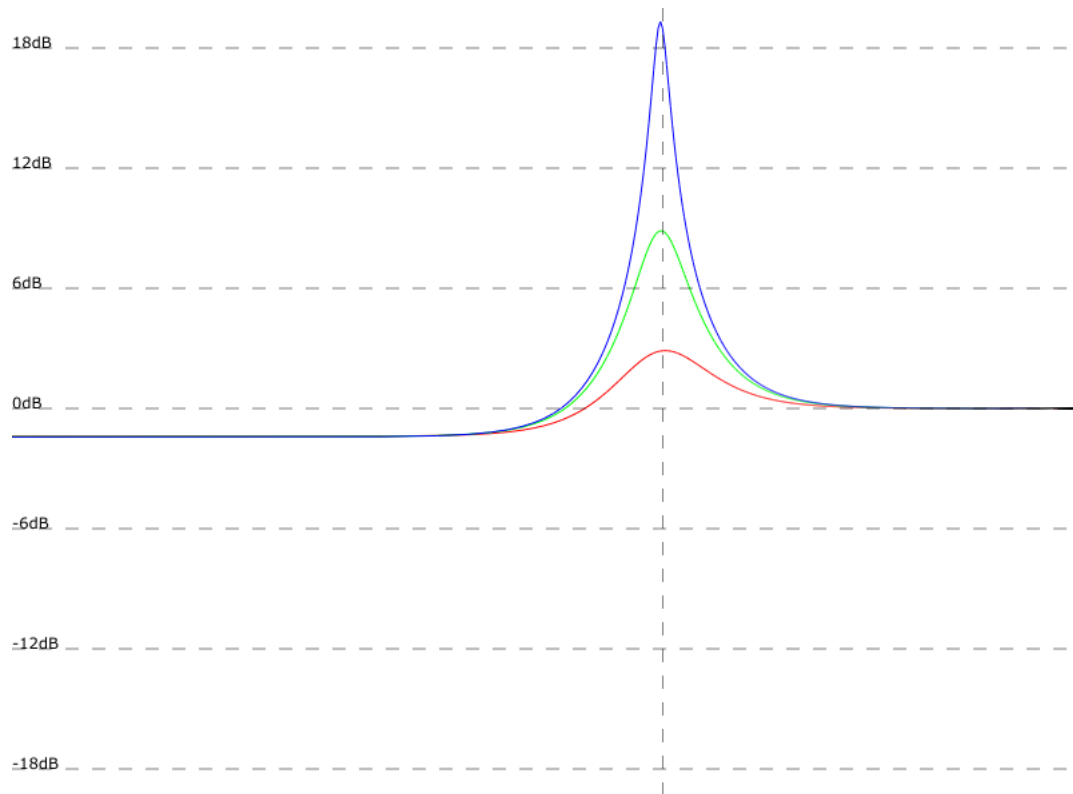
Figure 17. Peak filter response.
