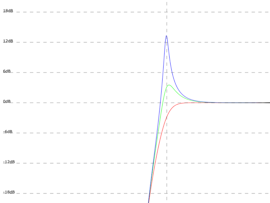
Figure 13. Highpass filter response.
