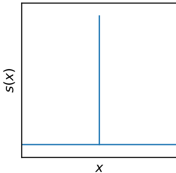
CEDT ( \varepsilon = 0 )
