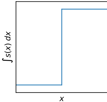
CEDT ( \varepsilon = 0 )
