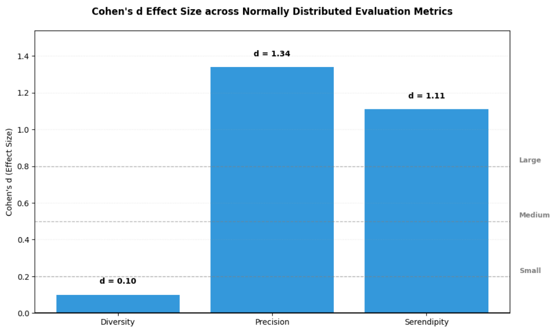
Figure 6.8: The Cohen effect size, d , of our three normally-distributed evaluation metrics.
