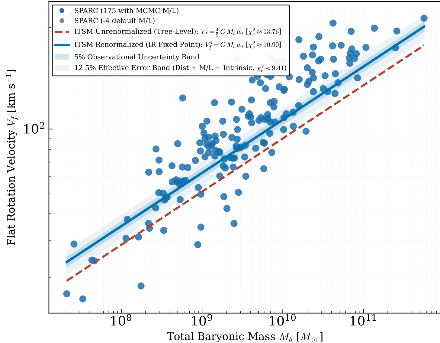
ITSM Baryonic Tully-Fisher Relation Renormalization Group Vertex Flow: g_0^2 = 4/9 \rightarrow g^{*2} = 1.0
