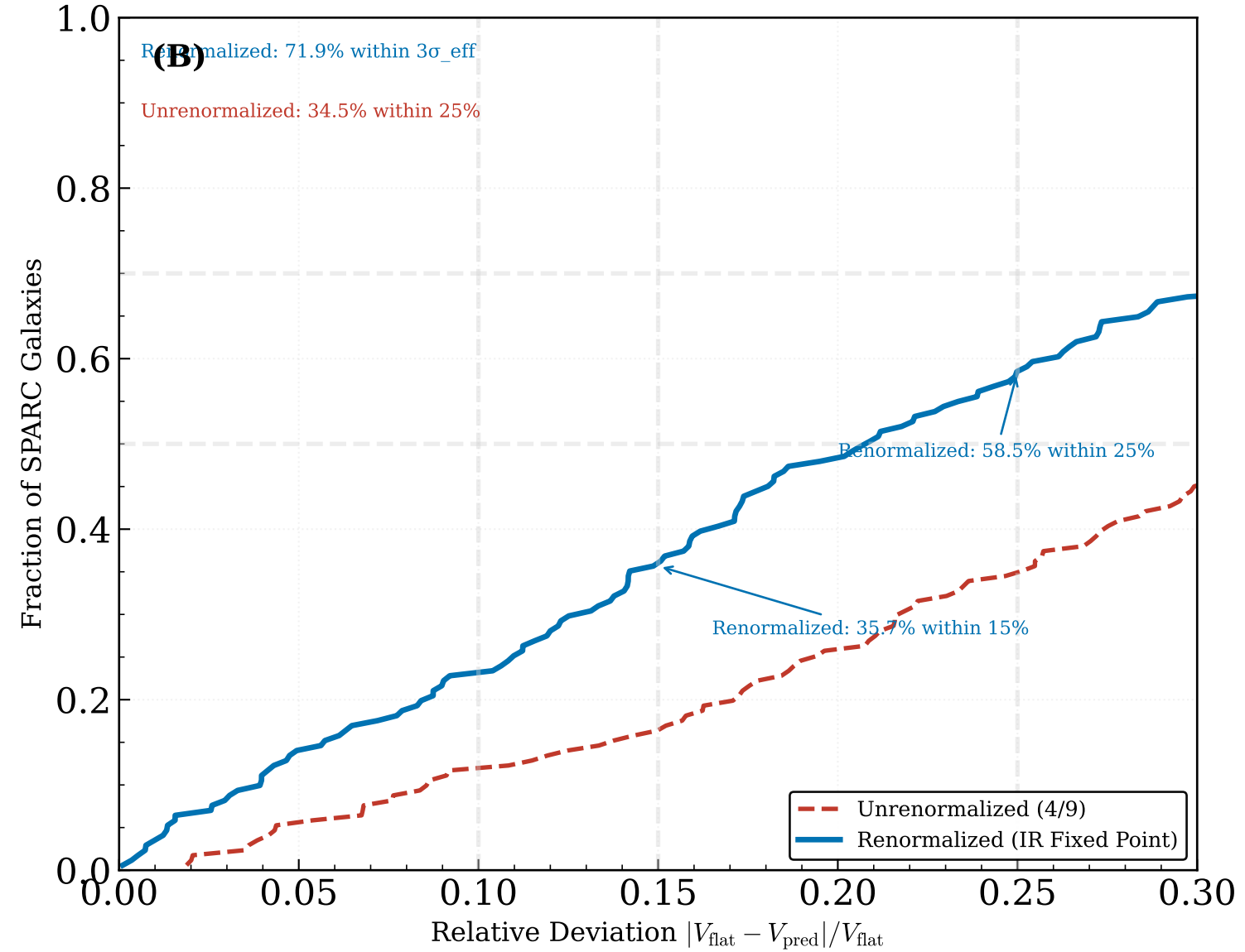
Cumulative Residual Distribution 171 SPARC Galaxies
