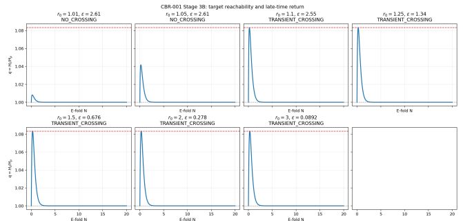
FIG. 3. Representative Stage-3B trajectories of q = H_t/H_p versus N . The horizontal line marks 13/12. Passages, when present, are brief; late evolution returns to isotropy.
