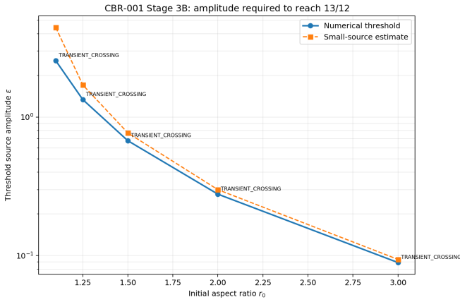
FIG. 4. Stage-3B threshold amplitudes \epsilon_*(r_0) for first touch of q = 13/12 . Near-cubic shapes require large source-scale ratios; no threshold defines an attractor.
