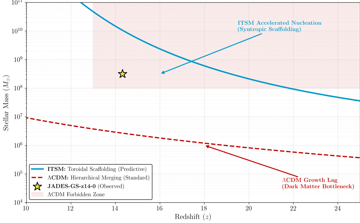
FIG. 8. Baryonic mass assembly history for JADES-GS-z14-0 ( z = 14.32 , t_{\text{age}} \approx 290 Myr). The \Lambda CDM hierarchical merging model (dashed red) cannot accumulate M_{\star} \gtrsim 10^{8.5} M_{\odot} within the available cosmic time, establishing a high-mass forbidden zone (shaded). The ITSM toroidal scaffolding model (solid cyan) permits rapid baryonic condensation at pre-existing vacuum vortex cores, comfortably reaching the observed stellar mass threshold within the JWST-confirmed timeline.
