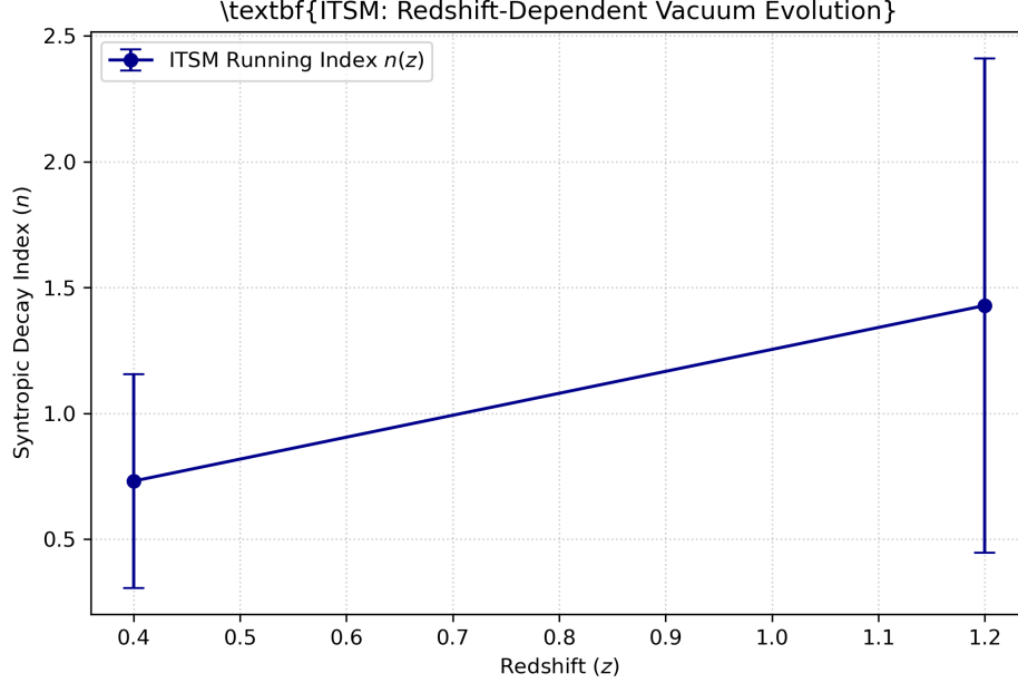
FIG. 11. ITSM Redshift-Dependent Vacuum Evolution. The shift from n \approx 0.71 to n \approx 1.45 identifies the Syntropic Decoupling Epoch.
