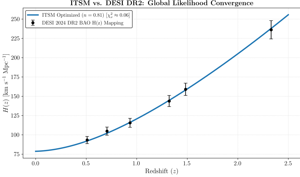
FIG. 10. ITSM optimized manifold confronting the DESI DR2 BAO consensus data ( H_0 = 78.63 \text{ km s}^{-1} \text{ Mpc}^{-1} ).
