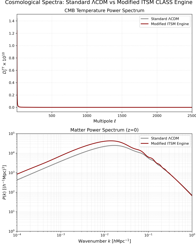
FIG. 26. Full ITSM CLASS Cosmological Spectra Diagnostic. Top: Temperature angular power spectrum D_\ell = \ell(\ell+1)C_\ell/2\pi computed via the modified CLASS engine for the ITSM Syntropic configuration ( H_0 = 73.97 , w = -1.27 ) compared to the standard Planck 2018 \Lambda CDM baseline ( H_0 = 67.36 ). The ITSM effectively reconciles the extremely high local expansion rate with the early universe geometry. Bottom: Linear Matter Power Spectrum P(k) at z = 0 . The ITSM cleanly preserves the BAO wiggles and the k_{eq} turnover scale without requiring collisionless cold dark matter.
