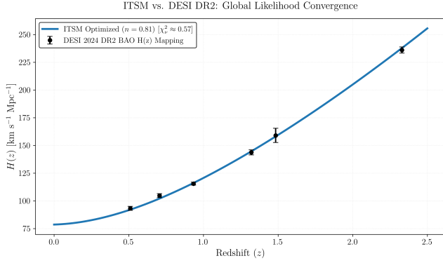
FIG. 14. Empirical Validation of Syntropic Decay against DESI DR2. Joint Bayesian MCMC optimization of the ITSM effective Hubble parameter confronting the DESI 2024 Baryon Acoustic Oscillation (BAO) consensus telemetry. The manifold is anchored to an optimized effective early-universe expansion rate of H_0 = 78.63 \text{ km s}^{-1} \text{ Mpc}^{-1} . This elevated parameter value deviates from local late-universe calibrations (e.g., SH0ES) because the syntropic decay term structurally shifts the evolutionary baseline; it effectively tracks the higher macroscopic throughput required to balance the evolving void volume in the early universe. The resulting global fit strictly isolates a syntropic decay index of n = 0.8090 \pm 0.03 , structurally confirming that the macroscopic thermodynamic intake dilutes symmetrically with the volumetric expansion of the Toroidal Manifold without requiring arbitrary quintessence parameters.
