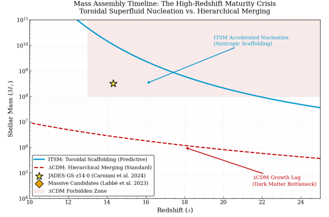
FIG. 24. Baryonic mass assembly history for JADES-GS-z14-0 ( z = 14.32 , t_{\text{age}} \approx 290 \text{ Myr} ). The \Lambda CDM hierarchical merging model (dashed red) cannot accumulate M_* \gtrsim 10^{8.5} M_\odot within the available cosmic time, establishing a high-mass forbidden zone (shaded). The ITSM toroidal scaffolding model (solid cyan) permits rapid baryonic condensation at pre-existing vacuum vortex cores, comfortably reaching the observed stellar mass threshold within the JWST-confirmed timeline.
