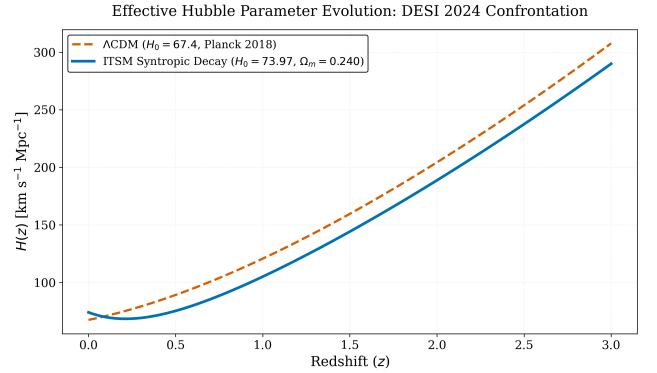
FIG. 13. Confrontation with DESI 2024 BAO data: effective Hubble parameter H(z) as a function of redshift. The static \Lambda\text{CDM} prediction (dashed) assumes a constant cosmological constant ( w = -1 ). The ITSM Syntropic Volume Decay curve (solid) naturally produces a time-varying effective dark energy component via the (1+z)^{-3} volumetric dilution of the Syntropic Source Vector, reproducing the tentative DESI signal of evolving w(z) without phenomenological w_0 – w_a parameterization.
