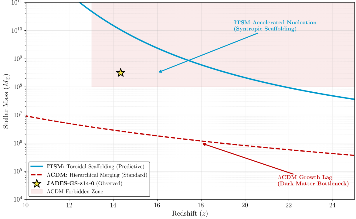
FIG. 9. Baryonic mass assembly history for JADES-GS-z14-0 ( z = 14.32 , t_{\text{age}} \approx 290 Myr). The \Lambda CDM hierarchical merging model (dashed red) cannot accumulate M_* \gtrsim 10^{8.5} M_\odot within the available cosmic time, establishing a high-mass forbidden zone (shaded). The ITSM toroidal scaffolding model (solid cyan) permits rapid baryonic condensation at pre-existing vacuum vortex cores, comfortably reaching the observed stellar mass threshold within the JWST-confirmed timeline.
