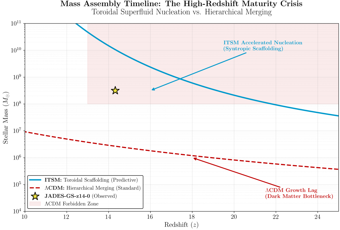
FIG. 8. Baryonic mass assembly history for JADES-GS-z14-0 ( z = 14.32 , t_{\text{age}} \approx 290 Myr). The \Lambda CDM hierarchical merging model (dashed red) cannot accumulate M_{\star} \gtrsim 10^{8.5} M_{\odot} within the available cosmic time, establishing a high-mass forbidden zone (shaded). The ITSM toroidal scaffolding model (solid cyan) permits rapid baryonic condensation at pre-existing vacuum vortex cores, comfortably reaching the observed stellar mass threshold within the JWST-confirmed timeline.
