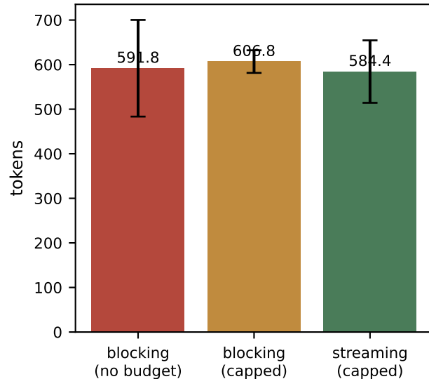
Tokens produced
