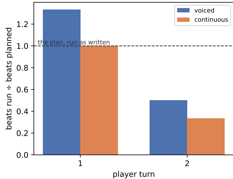
Plan adherence
