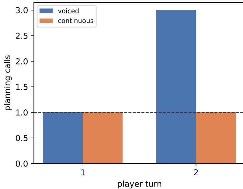
Planner calls per turn (target: 1)
