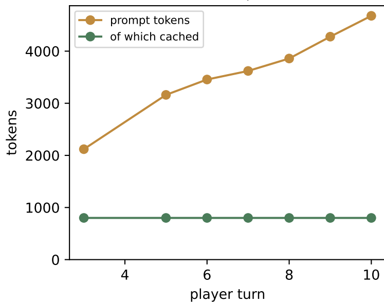
Context sent per turn
