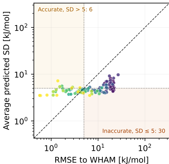
Optimized GP (LOO) ( r = 0.591 ) mean CRPS = 5.79 kJ/mol
