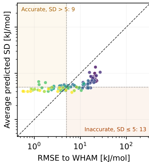
Hierarchical GP (LOO) ( r = 0.779 ) mean CRPS = 6.43 kJ/mol
