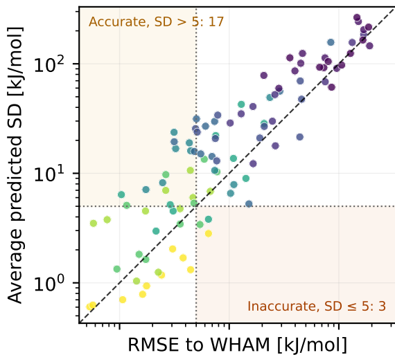
Optimized GP (LOO) ( r = 0.591 ) mean CRPS = 5.79 kJ/mol
