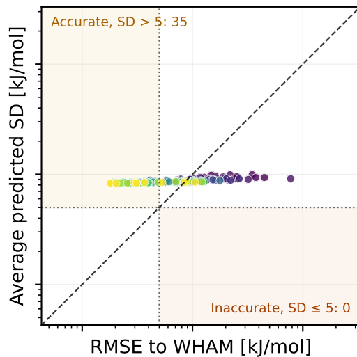
Hierarchical GP (LOO) ( r = 0.779 ) mean CRPS = 6.43 kJ/mol
