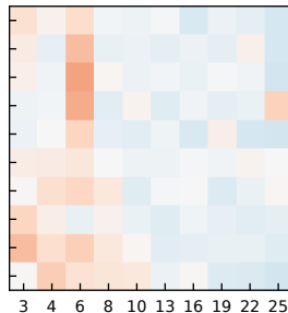
Number of umbrella windows
