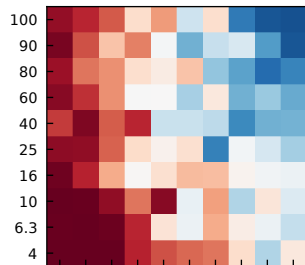
(a) Umbrella integration
