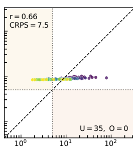
RMSE [kJ/mol]
