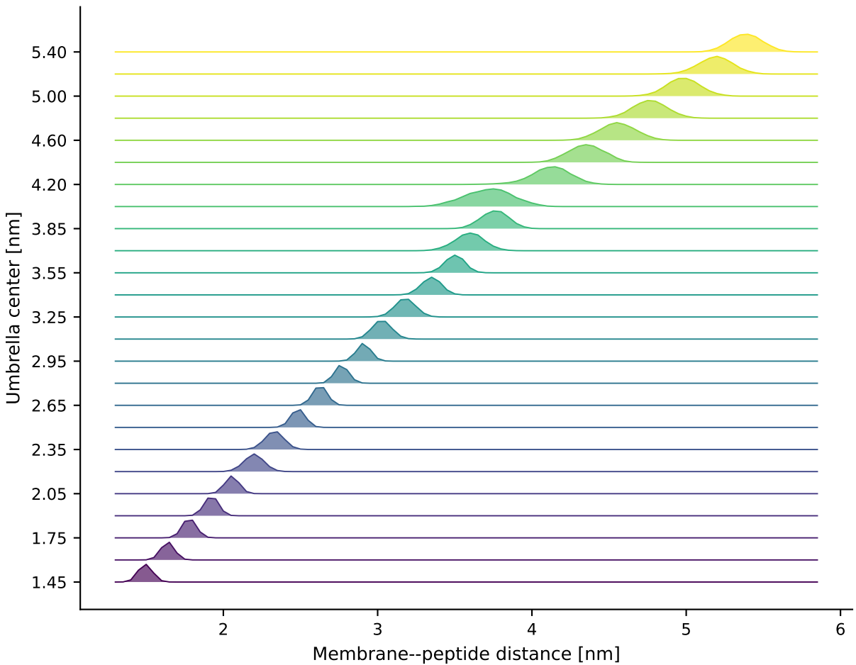
AR(1)-thinned full-data window histograms
