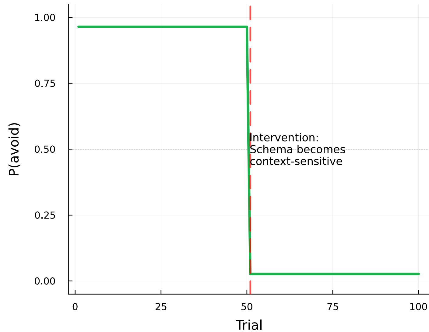
CT: Structural Change (Modularity-Breaking)
